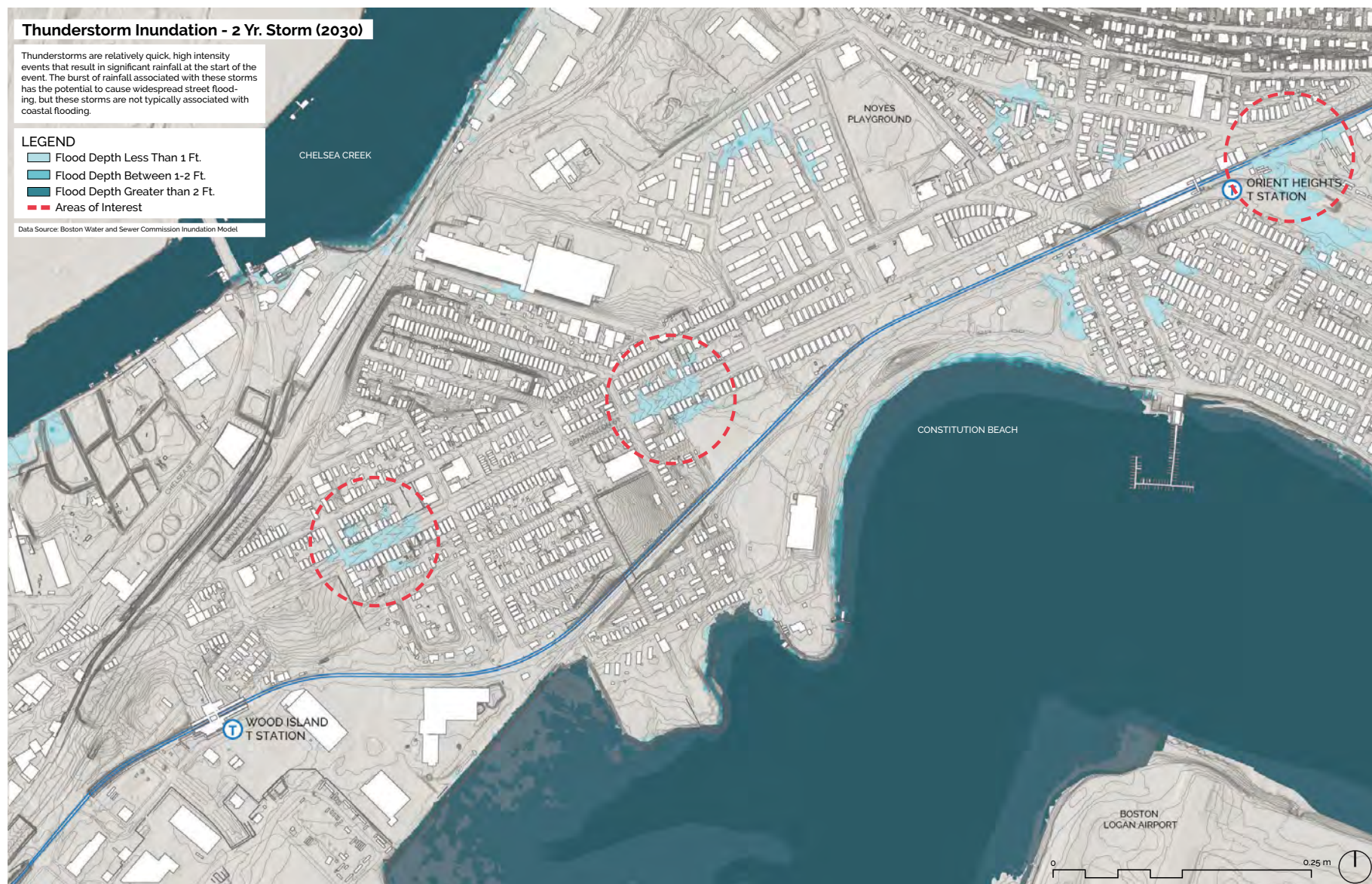
Thunderstorm Inundation - 2 Year Storm (2030) map created by Weston & Sampson (data source: Boston Water and Sewer Commission Inundation Model)
